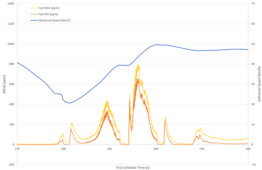
Figure 5: Moderate transients associated with more gentle gear changes
