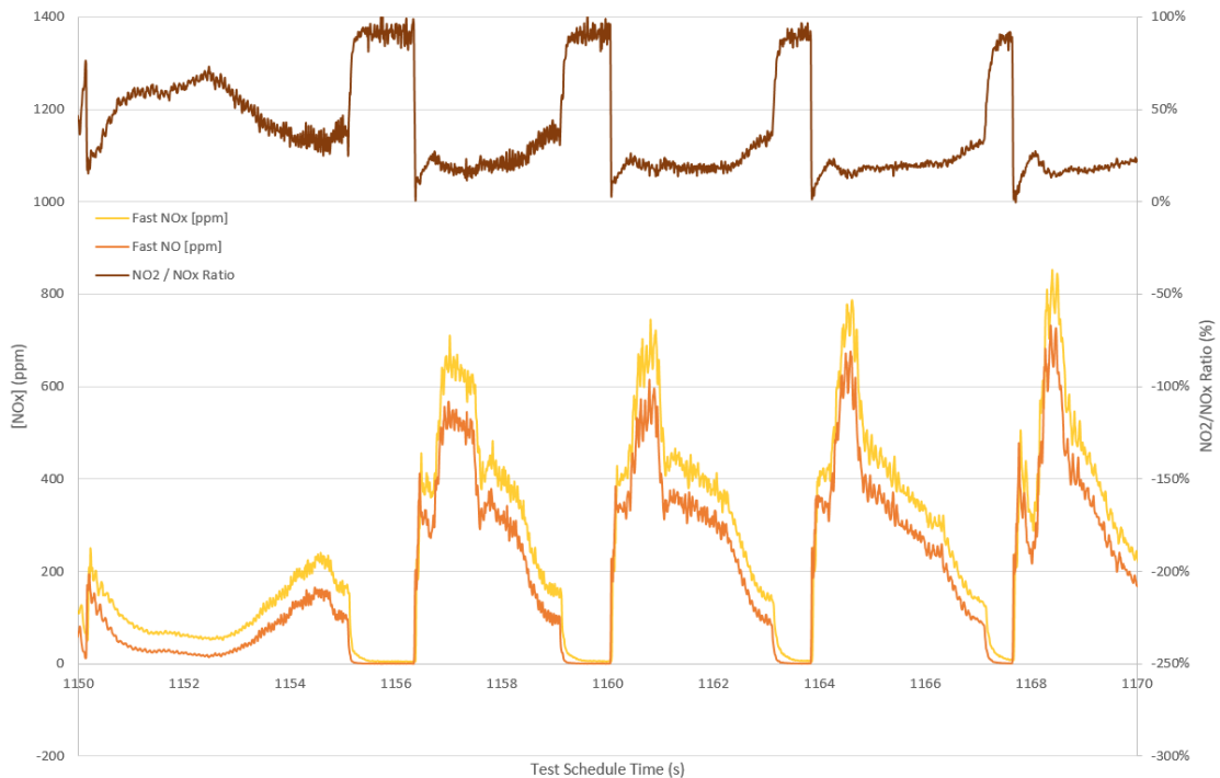
Figure 4: Transient NO x during hard accelerations and gear changes
