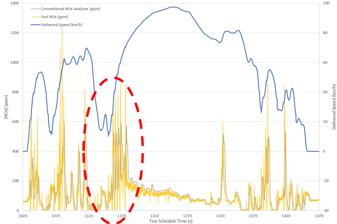
Figure 2: A portion of the highly transient WLTC drive cycle.
