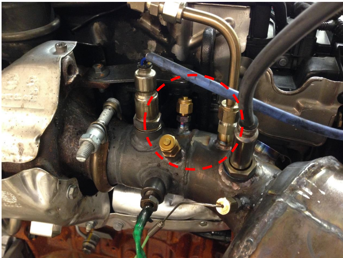
Figure 1: Engine-out sampling points for fast NO and NO x
