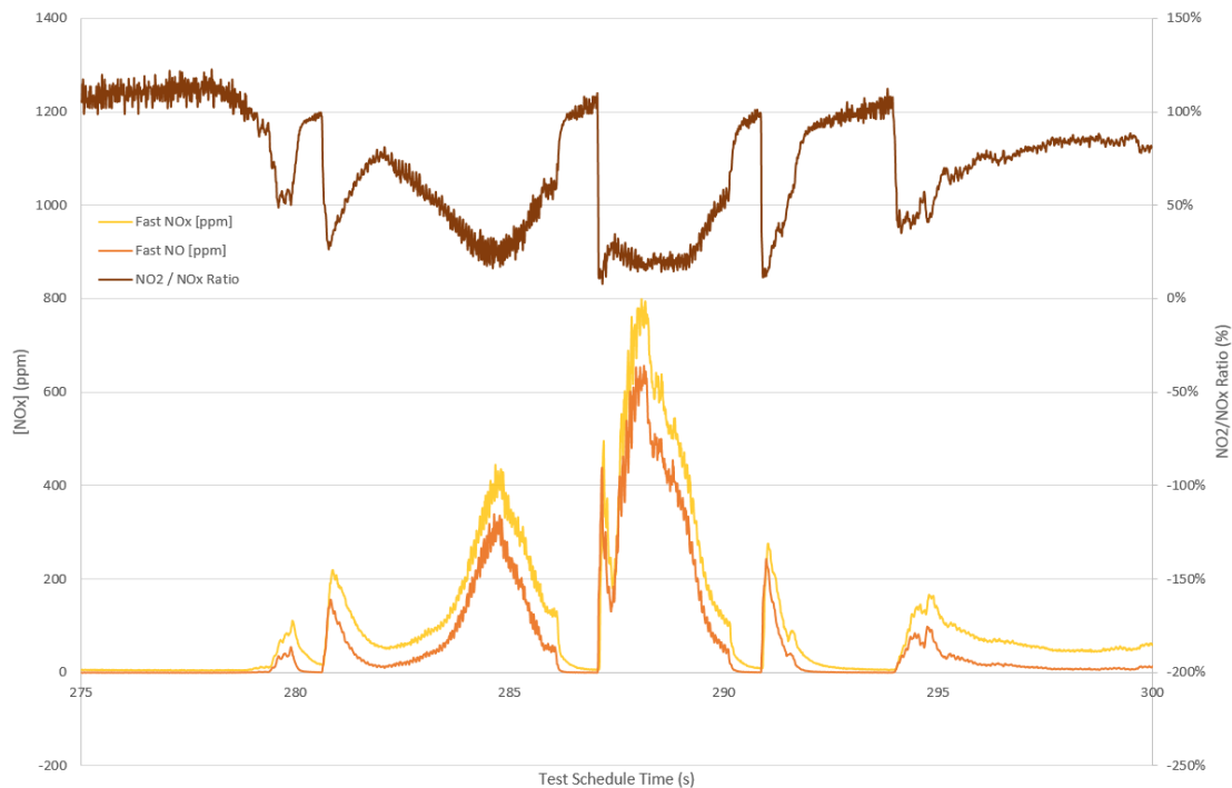
Figure 6: NO 2 : NO x ratio during moderate transients
