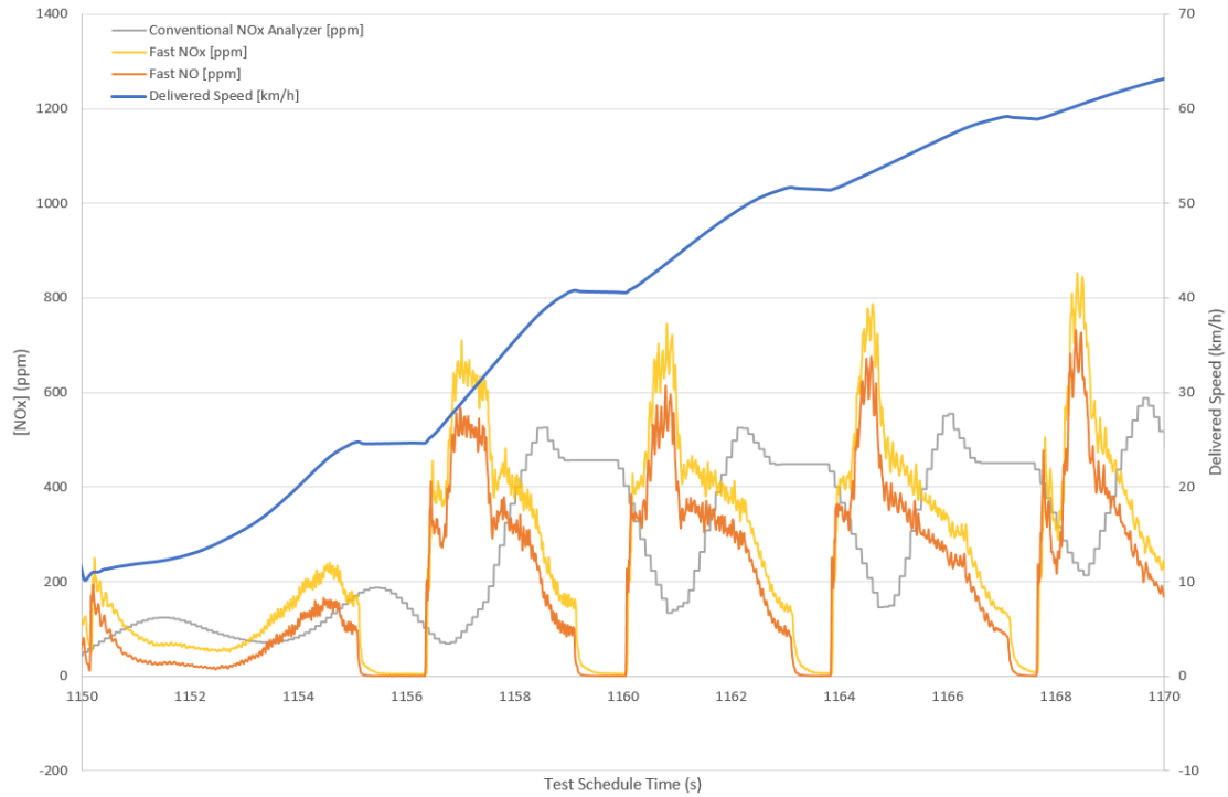
Figure 3: Detail of transient NO x during hard accelerations and gear changes compared with a conventional NO x analyzer
